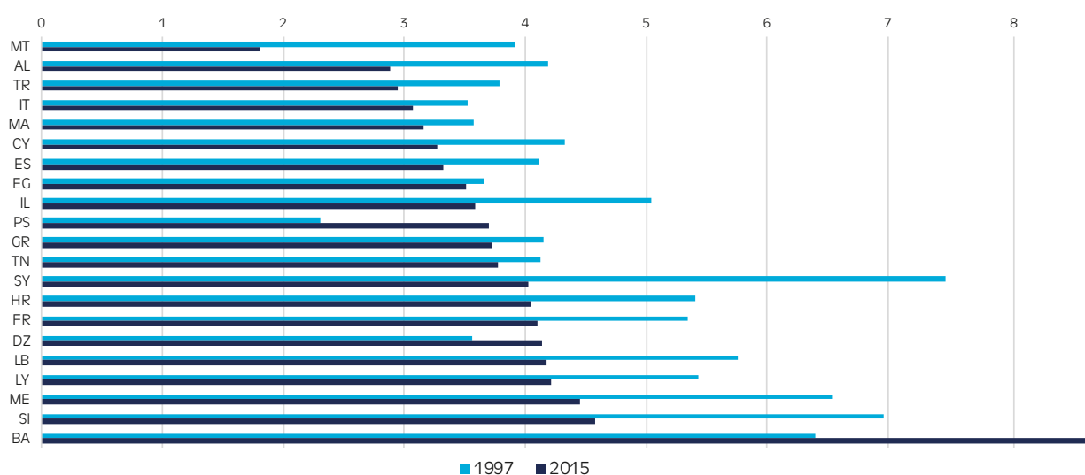
Figure 22 - Changes to energy intensity (ratio between energy supply and GDP at PPP) between 1997 and 2015 in MJ / GDP in USD 2011 PPP
