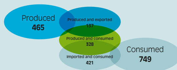
Figure 28 - Calculating the French carbon footprint, in millions of tons of CO 2 equivalent, 2017
